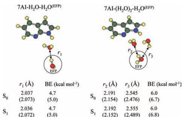
Figure 6. Geometries and binding energies of 7AI-H 2 O-H 2 O and 7AI-(H 2 O) 2 -H 2 O for which EFP results are compared with ab initio results. The numbers in parentheses denote ab initio values.
